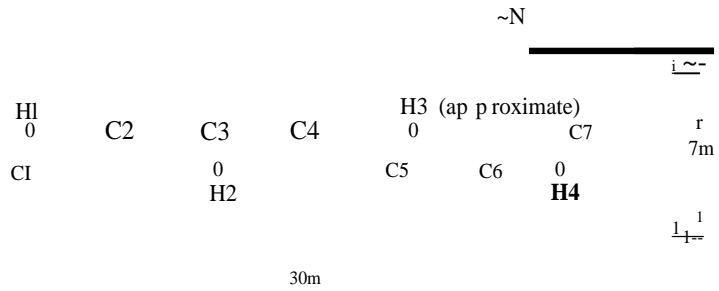
Figure 2a. Scheme of Crematorium II gas chamber from above. C1-C7 mark support pillars, H1-H4 Zyklon holes. Because roof shifted when dynamited, relative distances (e.g., between C1 and H1) differ today (see Figure 10 and relevant discussion).
